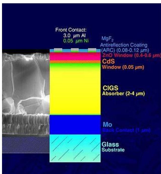
Figure 2: internal structure of Copper Indium diSelenide (CIS) Cells is shown
