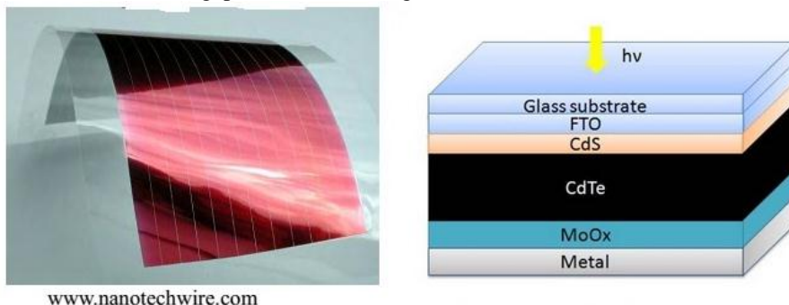
Figure 3: internal structure and general shape CdTe solar cell is shown.
